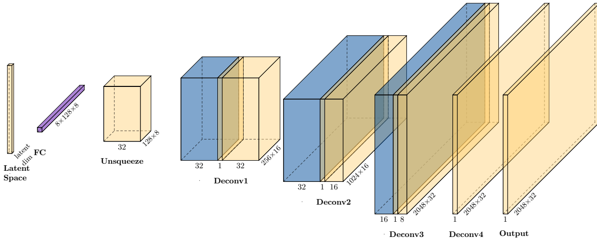
Figure 5.4: Architecture of the Efficient decoder. The input is a latent vector of dimension d . A fully connected layer first expands this into a feature map of size 8 \times 128 \times 8 , followed by a 1 \times 1 convolution ( Unsqueeze ) to increase the channel count to 32. The following three blocks ( Deconv1–3 ) each consist of nearest-neighbor upsampling and a depthwise-separable convolution: Deconv1 doubles both axes ( 32 \times 256 \times 16 ), Deconv2 restores horizontal resolution more aggressively with a 1 \times 4 upsampling ( 16 \times 1024 \times 16 ), and Deconv3 doubles both axes again to 8 \times 2048 \times 32 . The final block ( Deconv4 ) applies a (3 \times 17) convolution with circular padding along the azimuth, reducing the channels to 1 and producing the reconstructed output of size 1 \times 2048 \times 32 , which matches the original input dimensionality.
