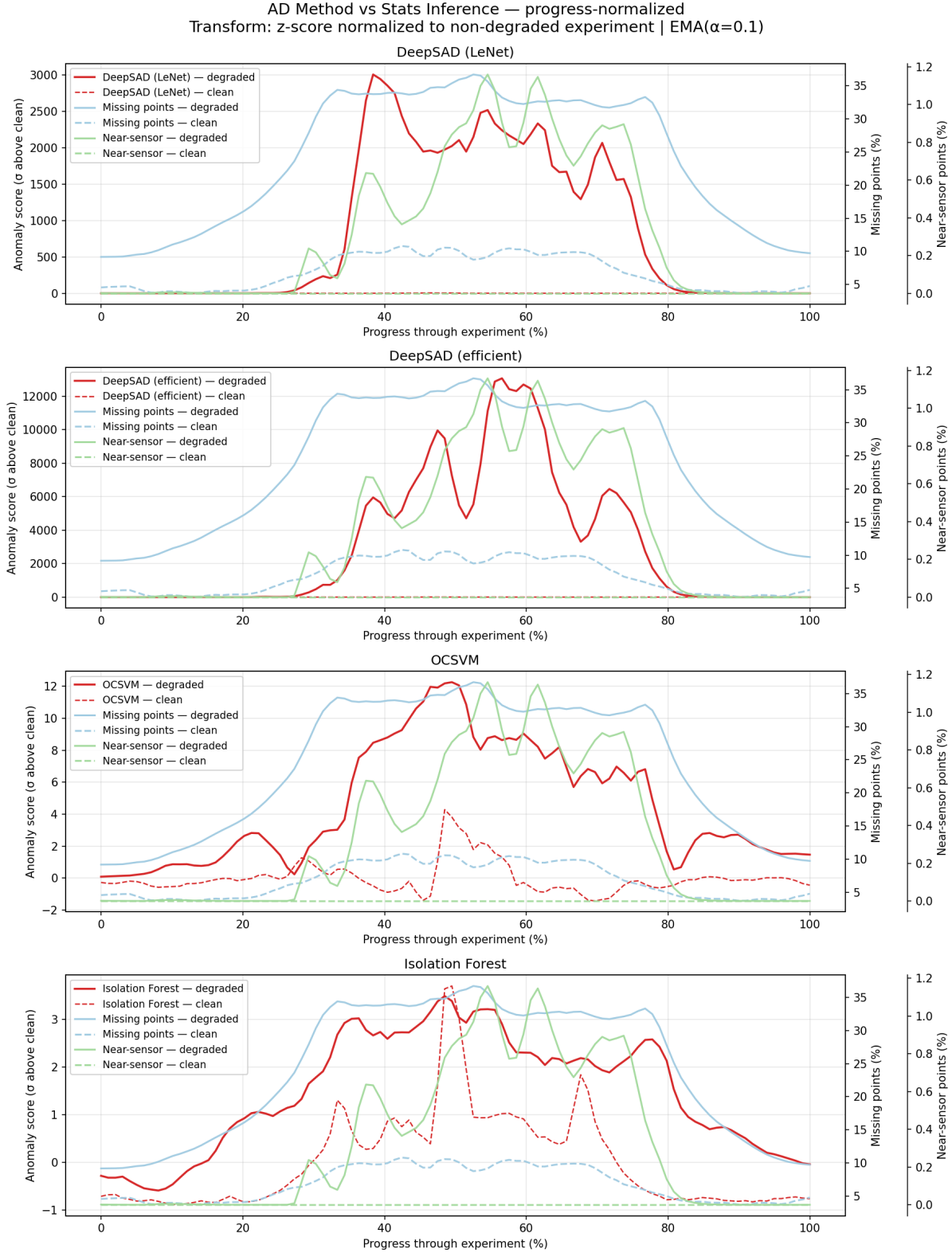
Figure 6.5: Comparison of anomaly detection methods with statistical indicators across clean (dashed) and degraded (solid) experiments. Each subplot shows one method (DeepSAD-LeNet, DeepSAD-Efficient, OCSVM, Isolation Forest). Red curves denote method anomaly scores normalized to the clean experiment; blue and green curves denote the percentage of missing LiDAR points and near-sensor particle hits, respectively. Clear separation between clean and degraded runs is observed for the DeepSAD variants and, to a lesser degree, for OCSVM, while Isolation Forest produces high scores even in the clean experiment. Latent Space Dimensionality was 32 and semi-supervised labeling regime was 0 normal and 0 anomalous samples during training.
