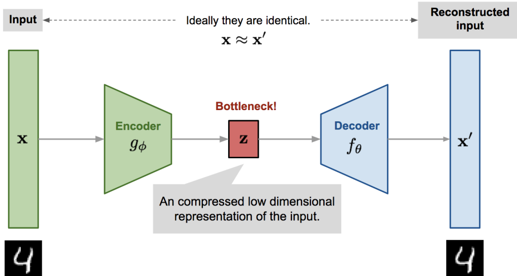
Figure 2.3: Illustration of an autoencoder's working principle. The encoder g_\phi compresses the input into a lower-dimensional bottleneck representation z , which is then reconstructed by the decoder f_\theta . During training, the difference between input and output serves as the loss signal to optimize both the encoder's feature extraction and the decoder's reconstruction. Reproduced from [17].
