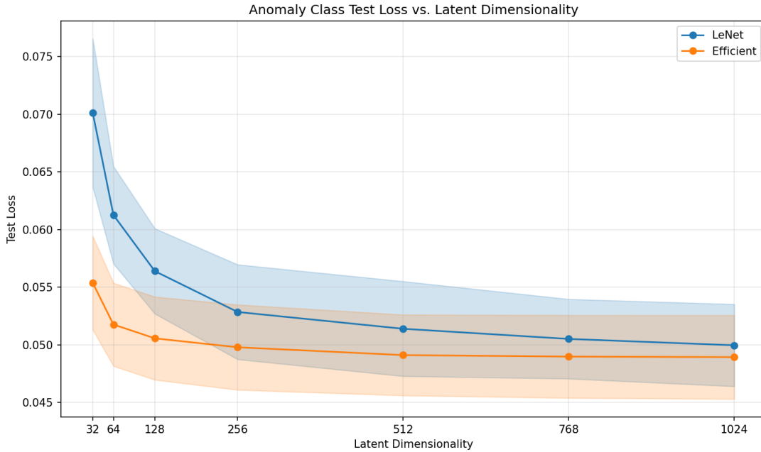
Figure 6.2: Reconstruction loss across latent dimensions for LeNet-inspired and Efficient autoencoder architectures, evaluated only on degraded data from manually-defined smoke experiments.
