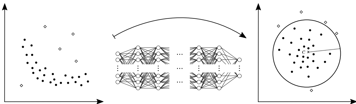
Figure 3.1: DeepSAD teaches a neural network to transform data into a latent space and minimize the volume of an data-encompassing hypersphere centered around a predetermined centroid c . Reproduced from [16].
