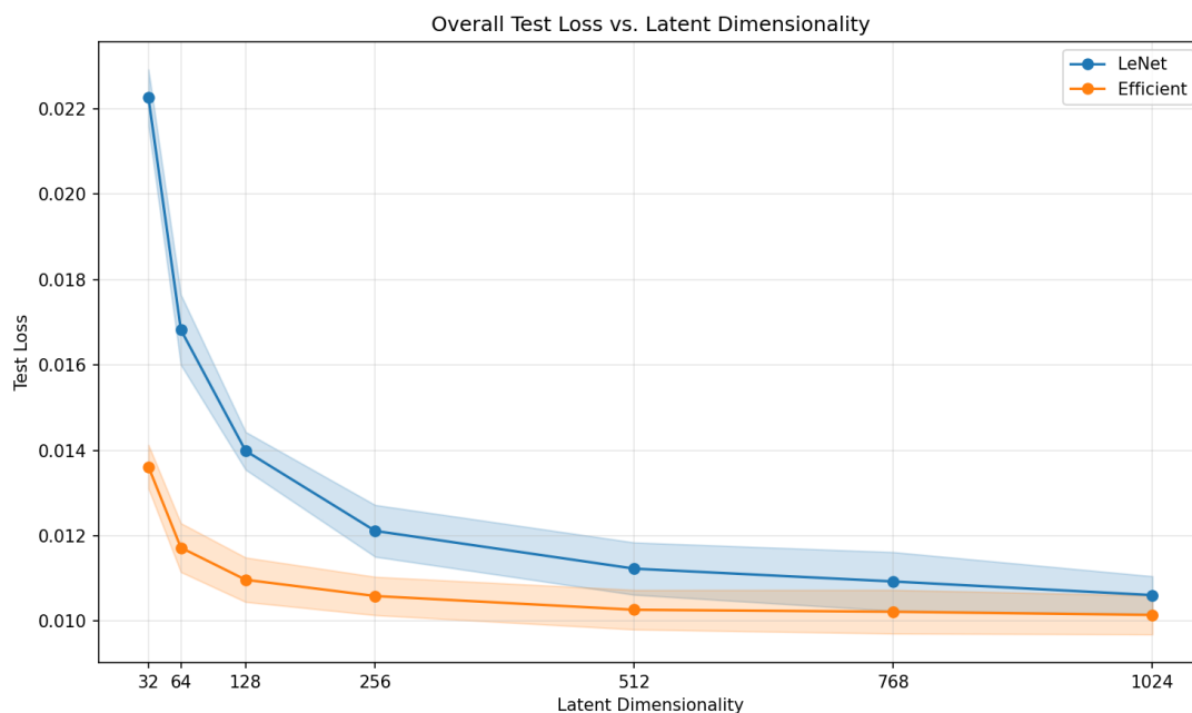
Figure 6.1: Reconstruction loss across latent dimensions for LeNet-inspired and Efficient autoencoder architectures.
