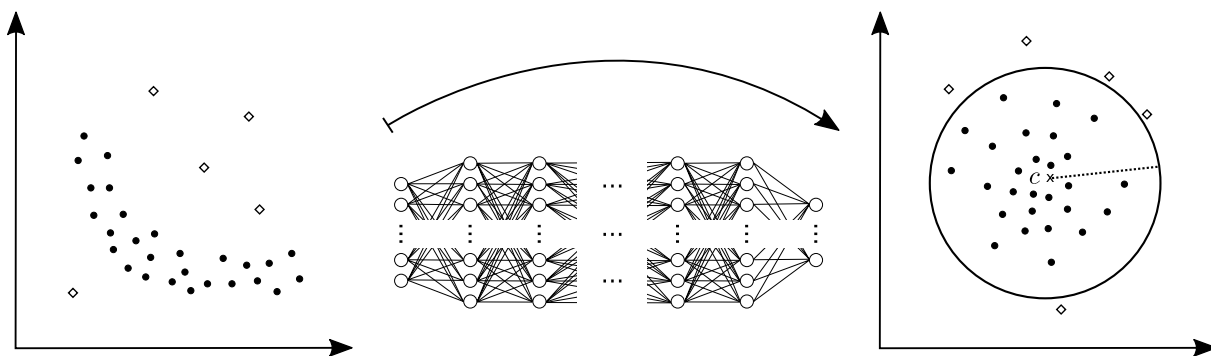
Figure 3.1: DeepSAD teaches a neural network to transform data into a latent space and minimize the volume of an data-encompassing hypersphere centered around a predetermined centroid c . Reproduced from [16].
