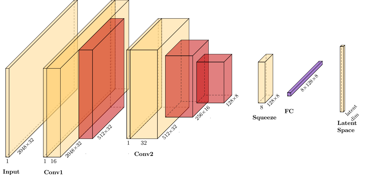
Figure 5.4: Architecture of the Efficient encoder. The input is a LiDAR range image of size 1 \times 2048 \times 32 (channels \times width \times height). The first block ( Conv1 ) applies a depthwise-separable 3 \times 17 convolution with circular padding along the azimuth, followed by batch normalization, LeakyReLU, and an aggressive horizontal pooling step, producing an intermediate representation of 16 \times 512 \times 32 . The second block ( Conv2 ) applies another depthwise-separable convolution with channel shuffle, followed by two stages of 2 \times 2 max pooling, yielding 32 \times 128 \times 8 . A 1 \times 1 convolution ( Squeeze ) then reduces the channel dimension to 8, producing 8 \times 128 \times 8 . Finally, a fully connected layer ( FC ) flattens this feature map and projects it into the latent space of size d , where d is a tunable hyperparameter ( 32 \leq d \leq 1024 in our experiments).
